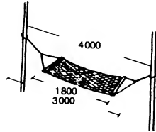
6 Hammock
